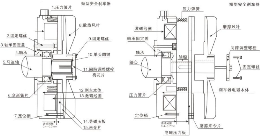
剎車間隙調整 ( AD JUST BRAKE CLEARANCE)
