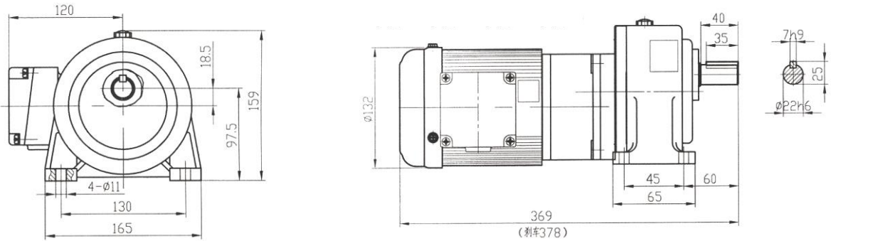
CH28+CH18-100-250~1800
