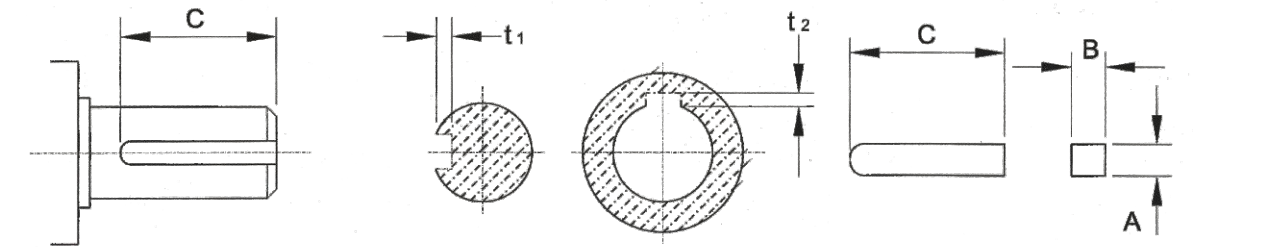
鍵/鍵槽加工尺寸 (KEY/KEY WAY DIMENSION)
