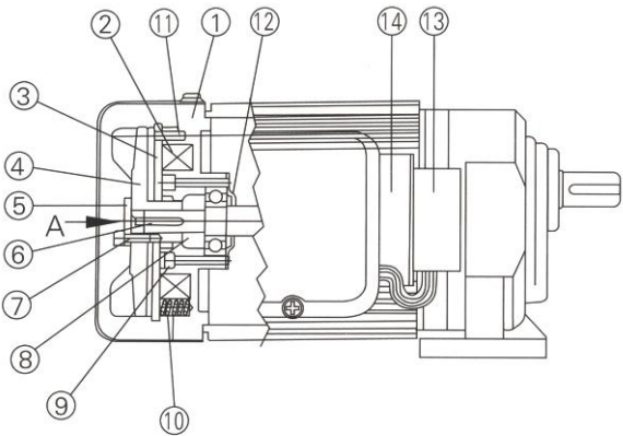
剎車裝配圖 Braking assembly drawing
